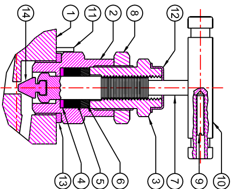
BONNET ASSEMBLY
